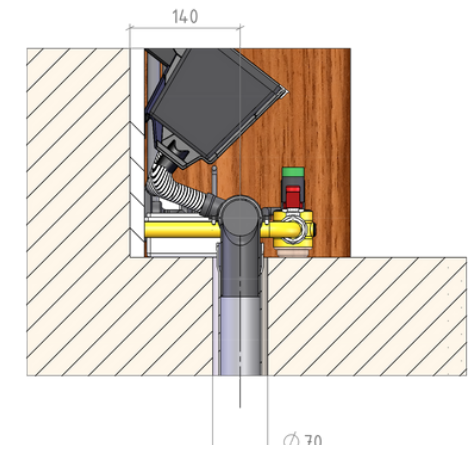
B Drain detail - DN50
