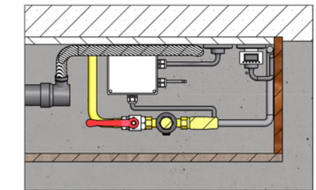
C-C Detail of control system (1:7)
