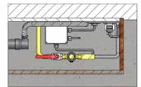
C-C Detail of control system (1:7)
